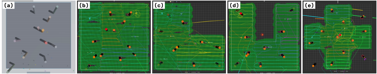
FIGURE 7. (a) Gazebo, rect scenario (screenshot); (b)–(e) final RViz coverage maps (green) of the PID- H_\infty missions, from the recordings ( https://youtube.com/playlist?list=PLfxyCAwHmhHI ).
